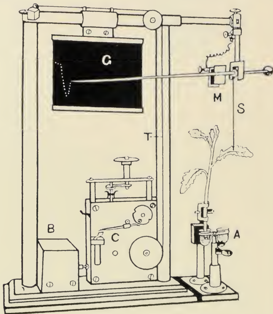
FIG. 7. The Electro-Magnetic Phytograph.
